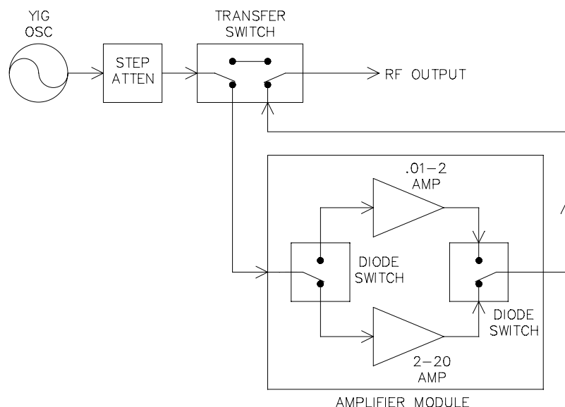
Figure A-1. Switches and Amplifiers for Option 20
