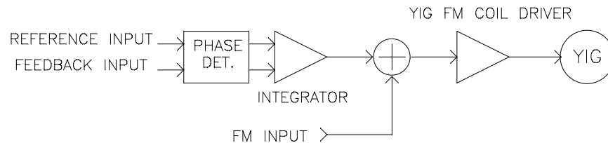
Figure 3-10. Frequency modulation
