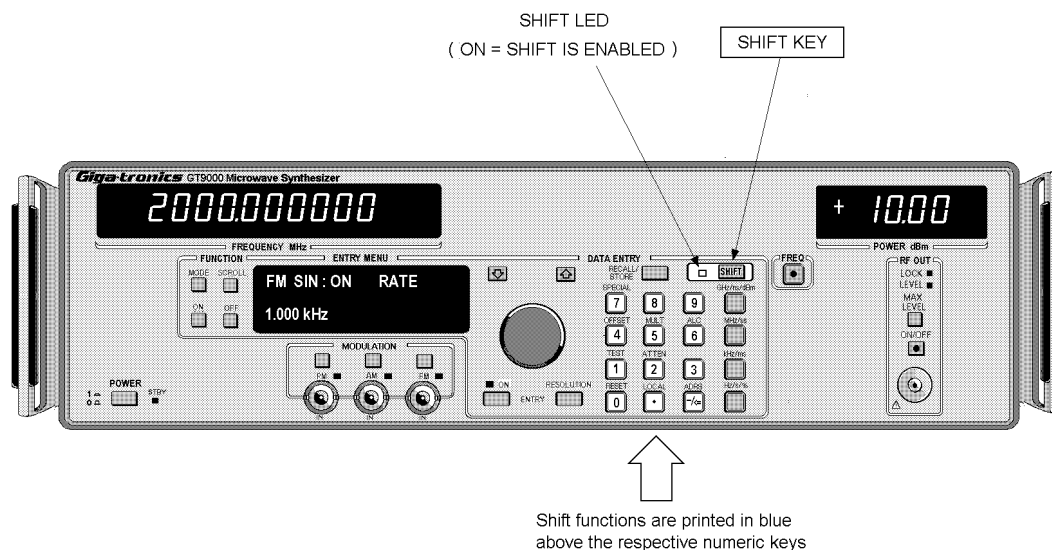
Figure 2-4. Shifted Functions
