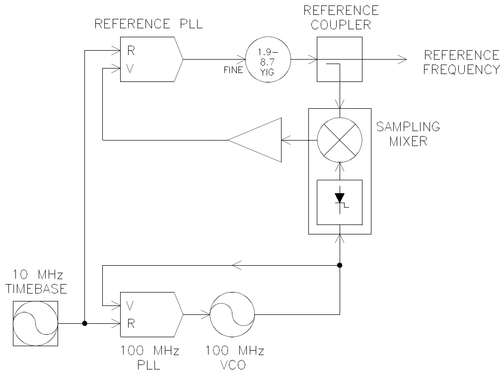
Figure 3-6. The reference loop
