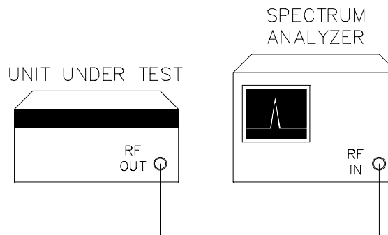
Figure 4-3. Single-Sideband Phase Noise
