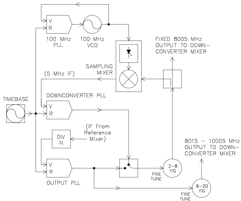
Figure 3-8. Downconverter phase lock loop
