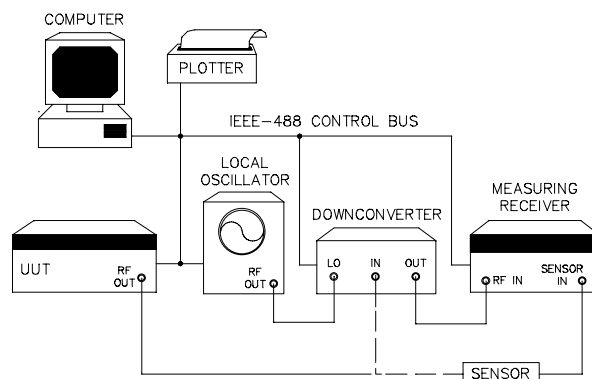
Figure 4-4. RF Output Power Tests
