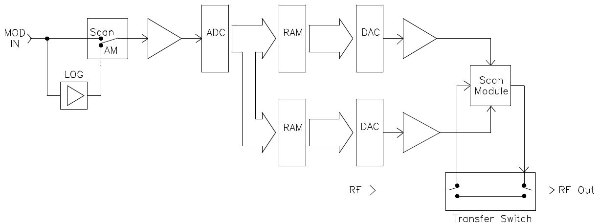
Figure A-3. Scan Modulation
