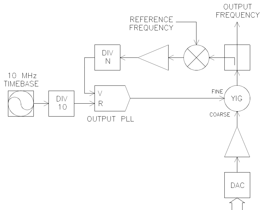
Figure 3-5. The output loop
