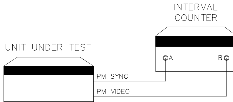
Figure 4-9. Internal Pulse Generator Tests
