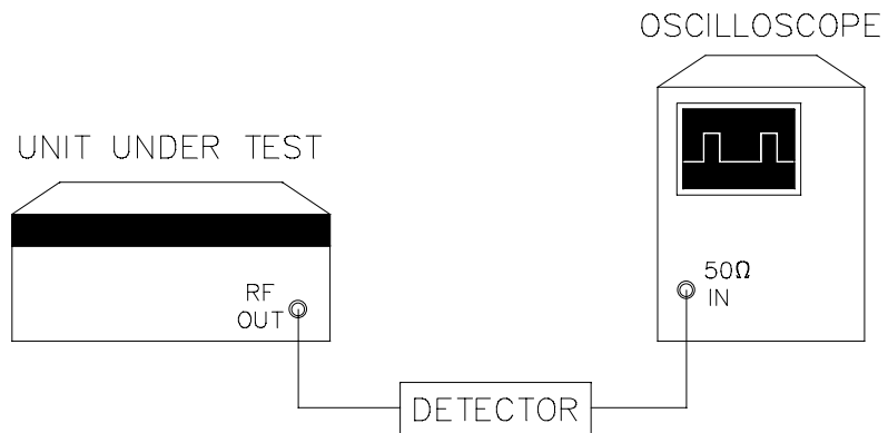
Figure 4-7. PM Overshoot & Settling Time
