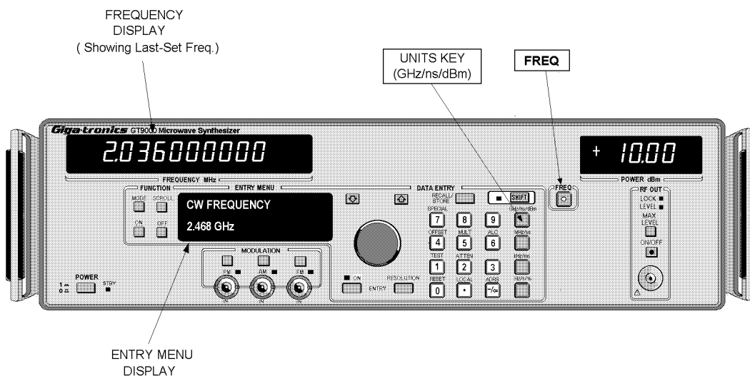
Figure 2-5. CW Frequencies
