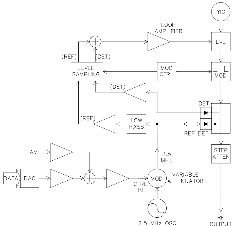
Figure 3-9. Automatic level control & AM
