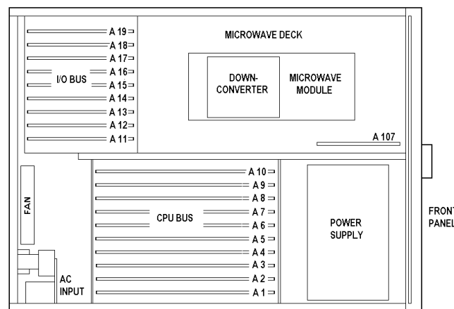
Figure 3-1. Internal Chassis Layout
