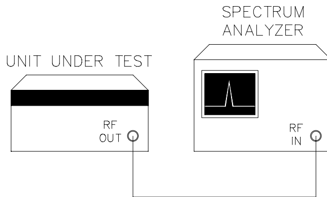
Figure 4-5. Pulse Modulation On/Off Ratio Test
